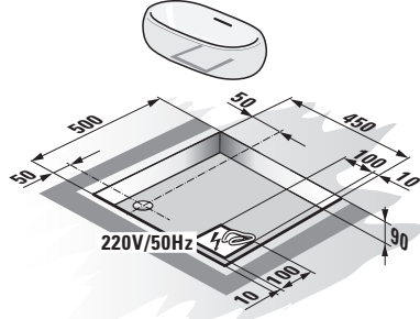
Positions for waste and power supply in the floor cut out
